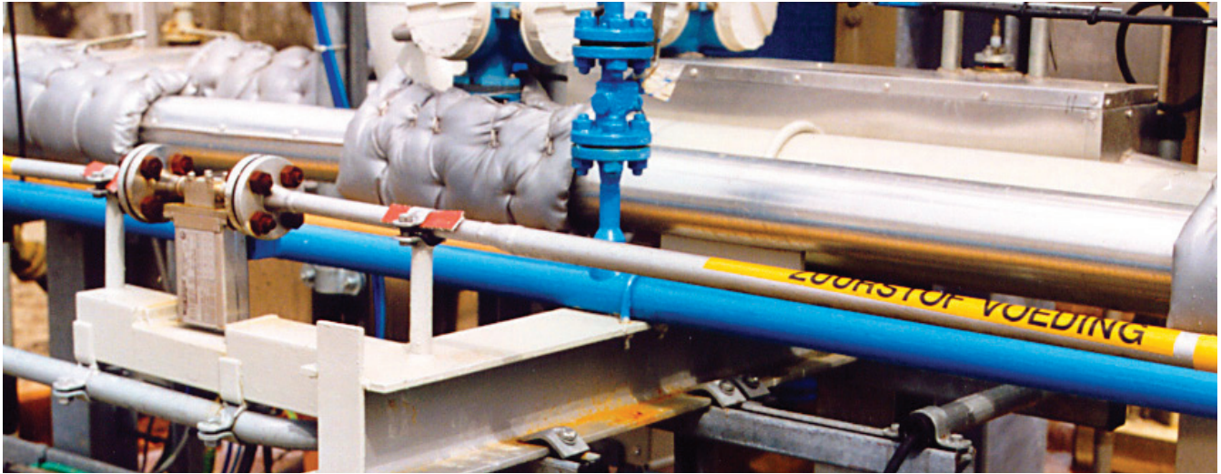
Oxygen Measurement
