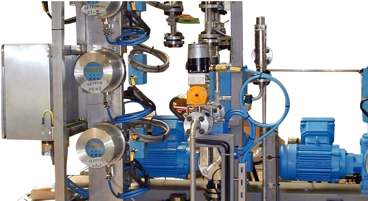
Oil & Gas flow metering skid
